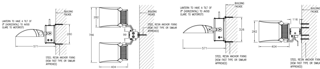
Single and double luminaire arrangement examples
