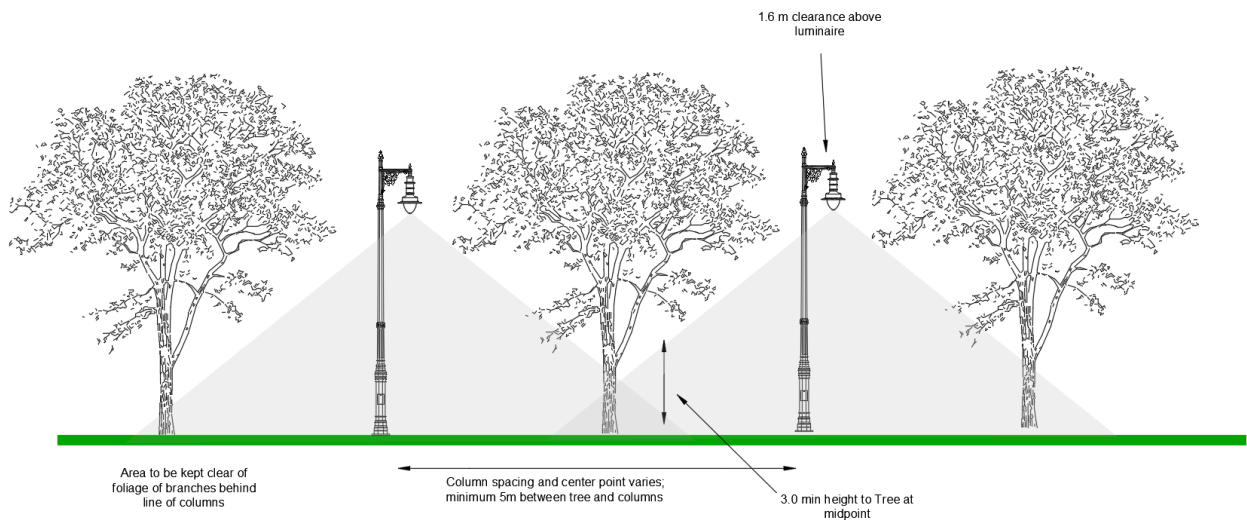
Areas to be maintained free of foliage and branches
