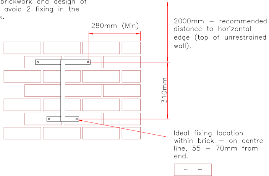
Indicative bracket anchor fixing example
