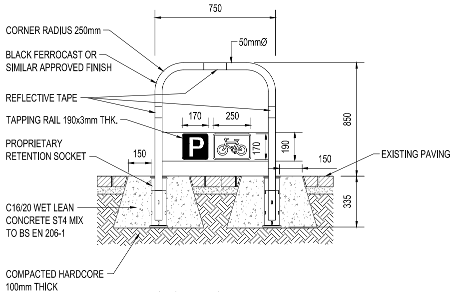
CYCLE RACK DETAIL TYPE 2
