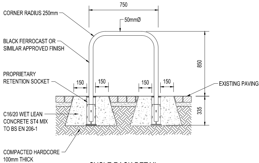
CYCLE RACK DETAIL TYPE 1
